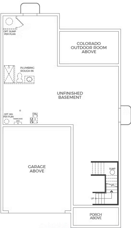
BASEMENT
