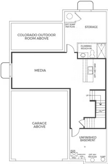
OPTIONAL FINISHED BASEMENT 1
