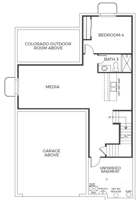
OPTIONAL FINISHED BASEMENT 2
