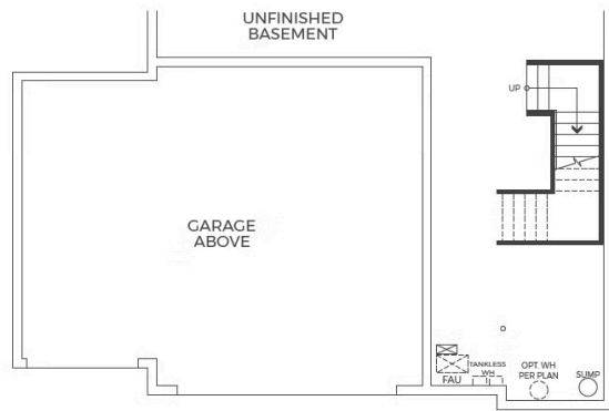
OPTIONAL 3-CAR GARAGE AT BASEMENT
