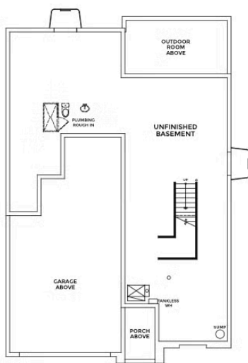
BASEMENT
