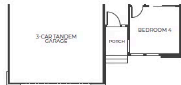
ELEVATION C FIRST FLOOR
