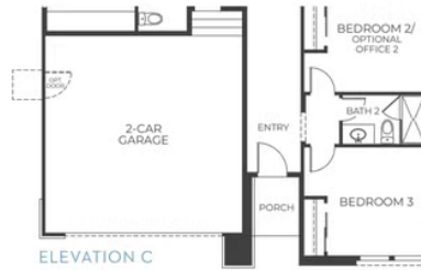
ELEVATION C FIRST FLOOR
