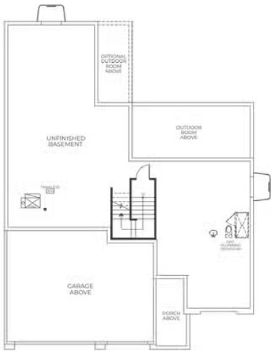
ELEVATION A BASEMENT
